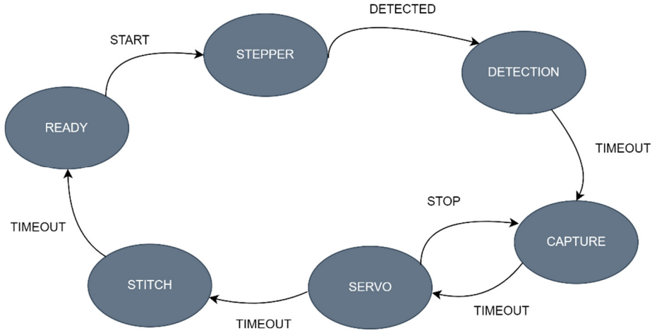
Figure 3 – System State machine
