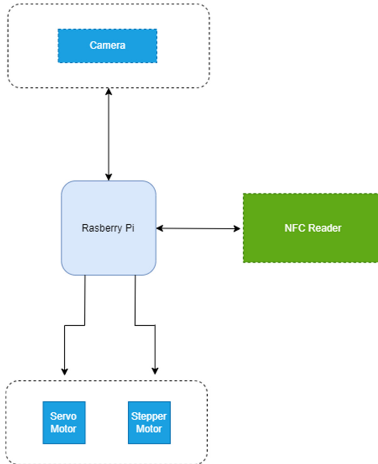
Figure 2 - Hardware overview
