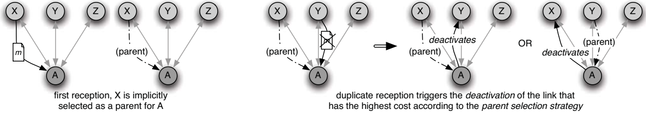
Fig. 3. Reception of a duplicate and deactivation of one link, for a tree BRISA structure. Depending on the parent selection strategy, the deactivated link can be the previous parent or the node sending the duplicate.
