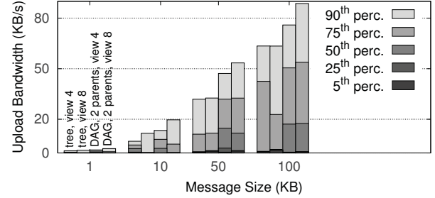
Fig. 11. Bandwidth usage for a 512 nodes network, upload.
