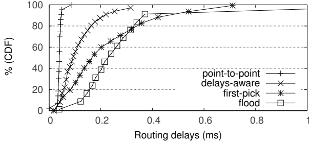
Fig. 9. Routing delays distribution on PlanetLab for a 150 nodes network. Structure is a tree with view size 4. Message size is 1KB×200 messages.
