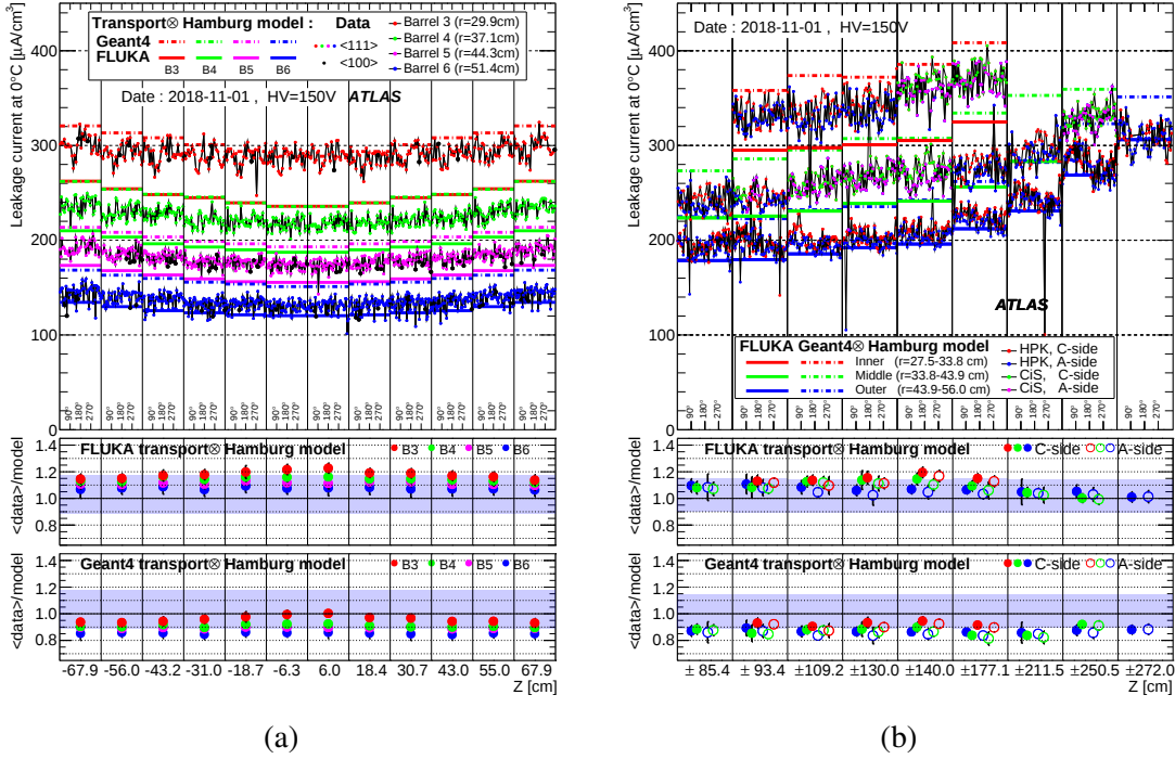
Figure 9. Leakage current measured at HV set to 150 V normalized to 0^\circ\text{C} per unit volume for all (a) barrel modules and (b) endcap modules as of November 1, 2018. At the same r and z location, modules with different \phi indices are arranged horizontally from left ( \phi = 0^\circ ) to right ( \phi = 360^\circ ). Endcap side-A and side-C as well as sensor manufacturers (Hamamatsu (HPK) and CiS) are plotted in different colours. Horizontal solid/dot-dash bars indicate model predictions of the Hamburg Model using the conversion factors by FLUKA (solid) / GEANT (dot-dash) transport simulations. In the two ratio plots, mean and RMS values via Gaussian fits of modules belonging to the same group are plotted. The model uncertainties are shown by blue bands.
