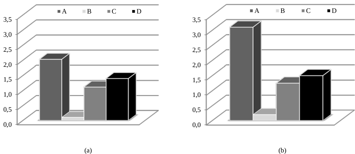
Figure 2 – Average exudation (%): (a) according to EN 445 (2007) three hours after mixing; (b) according to ASTM 940 (2010) 24h after mixing (except B). Product B had a fast setting and the test cannot be performed.
