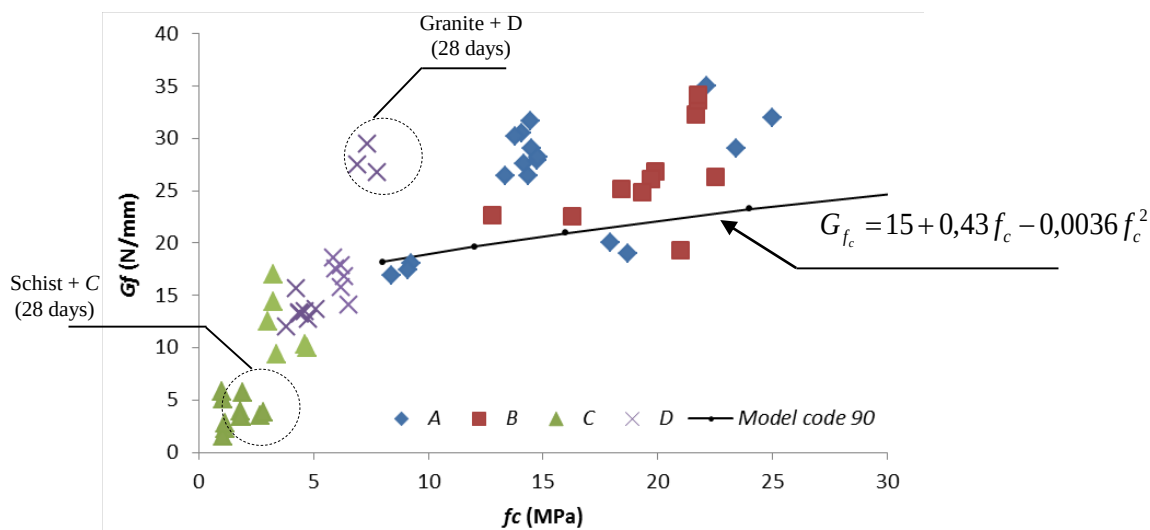
Figure 10 – Relationship between compressive strength ( f_c ) and fracture energy ( G_f )
