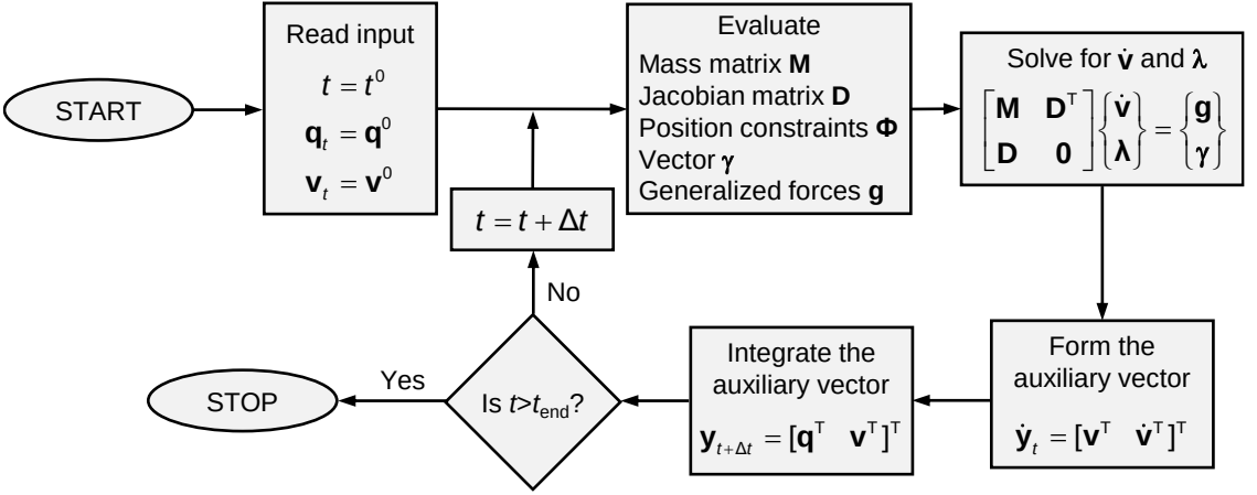
Figure 4. Flowchart of computational procedure for dynamic analysis of multibody systems.
