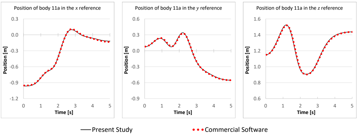
Figure 17. Comparison between the results for the forward kinematics of the robot's end-effector for the simulator utilized in the present study and a commercial software (Visual Nastran 4D).
