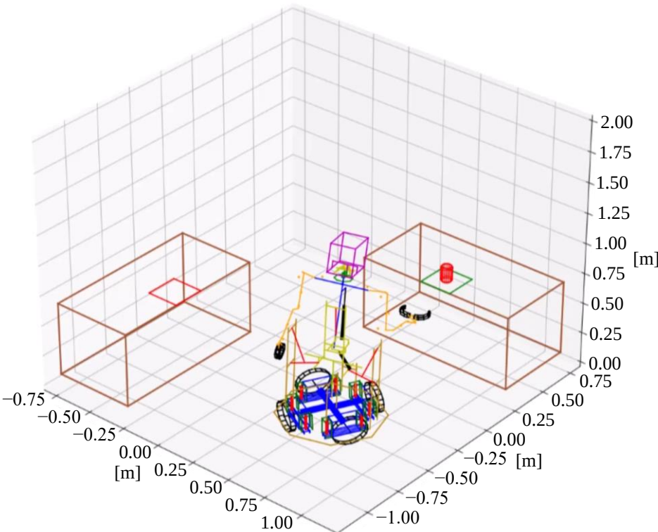
Figure 16. Simulation environment for testing the CHARMIE robot.
