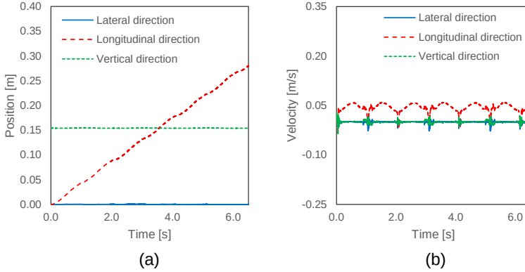
Figure 10. Global motion of the hexapod robot: (a) Position of the torso in the lateral, longitudinal and vertical directions; (b) Velocity of the torso in the lateral, longitudinal and vertical directions.
