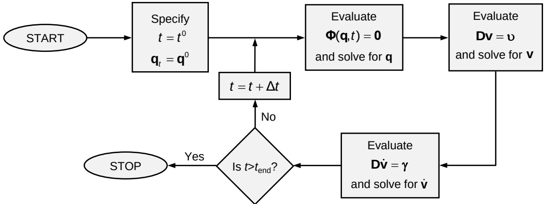
Figure 3. Flowchart of computational procedure for kinematic analysis of multibody systems.
