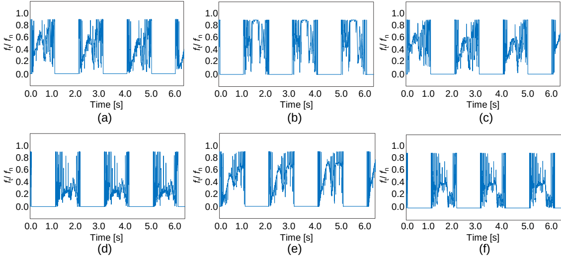
Figure 13. Plots of the hexapod robot's tangential contact forces: (a-f) Friction forces for limb 1 to 6.
