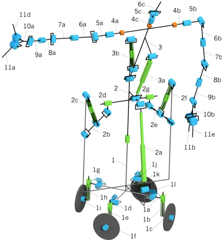
Figure 14. Kinematic diagram showcasing the bodies and degrees of freedom of the CHARMIE robot.
