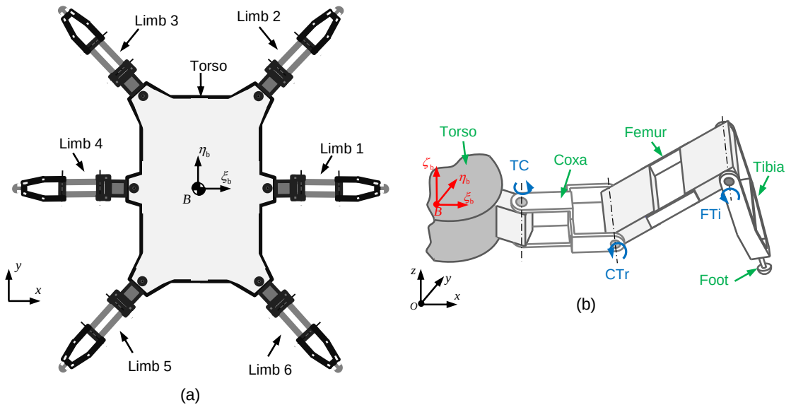
Figure 9. Hexapod robot multibody model: (a) Multibody subsystems; (b) Representation of each limb's multibody model: green identifies the system's rigid bodies, and blue represents the active joints.
