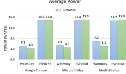
Fig. 7: Average power, in Watts, used by JS and Wasm on real-world applications.
