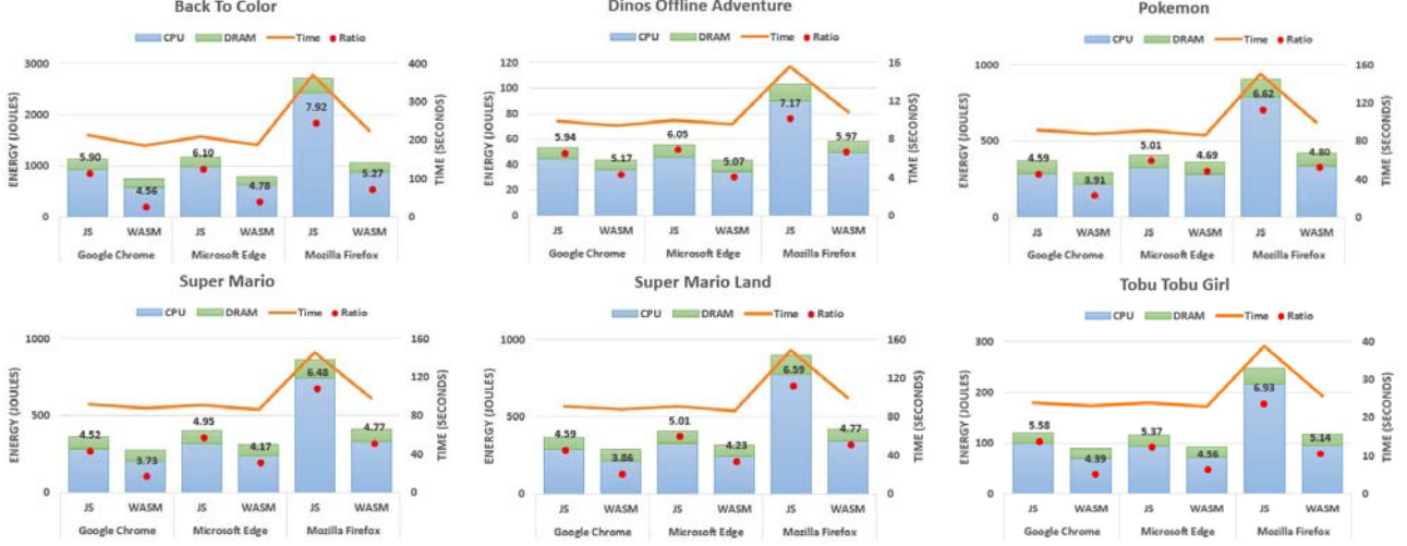
Fig. 1: WasmBoy : Energy consumed and run-time by each program in each Web browser.
