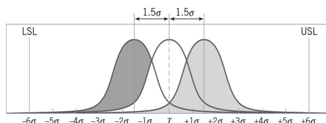
Figure 1. Normal distribution with the mean shifted by \pm 1.5\sigma [7].
