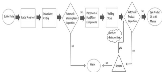
Figure 2. SMT Flowchart.
