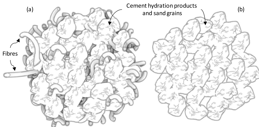
Figure 21. A schema of fibres filler mechanism in cement-based composites: (a) reinforced with fibres, (b) without fibres.
