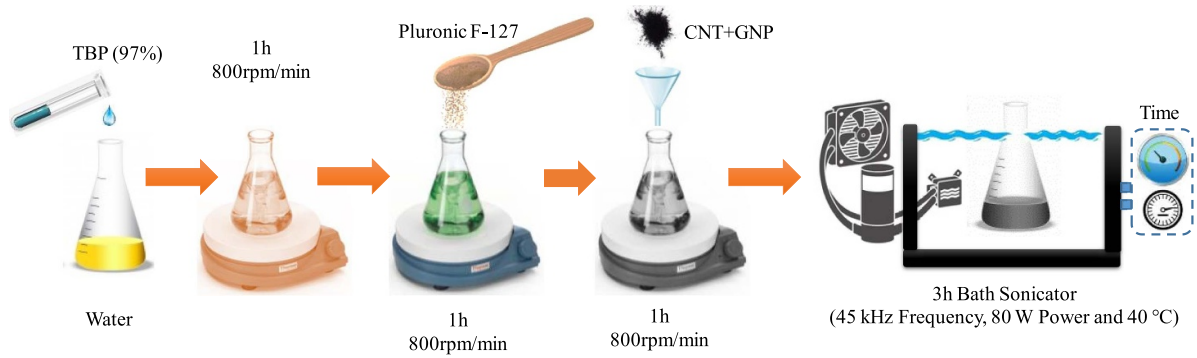
Figure 4. Dispersion methodology for CNMs employed in the study.
