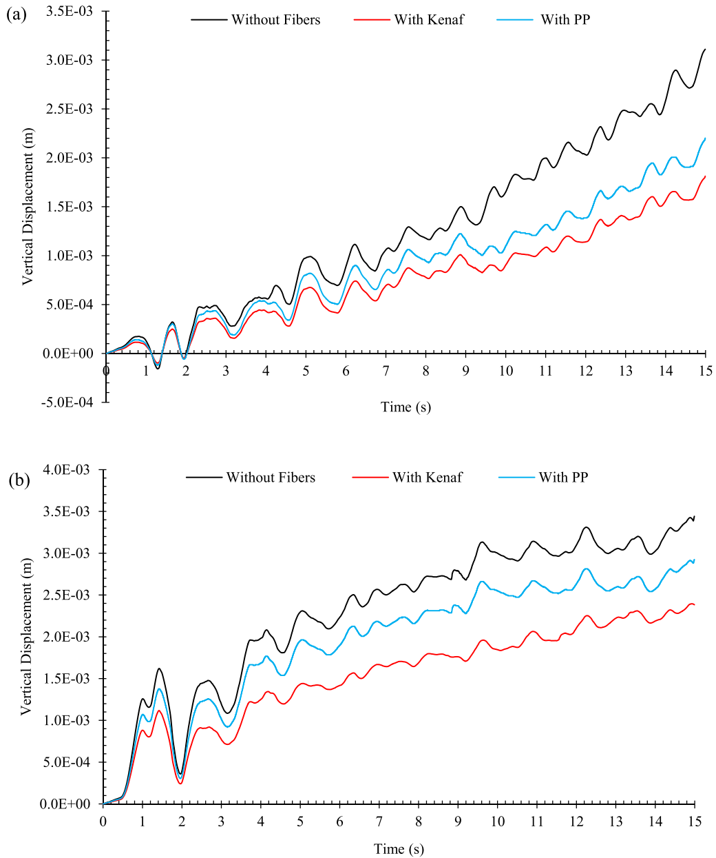
Figure 29. Vertical displacement curves of the tunnel shotcrete invert with different shotcrete types (uplift): (a) Tunnel 1 invert, (b) Tunnel 2 invert.
