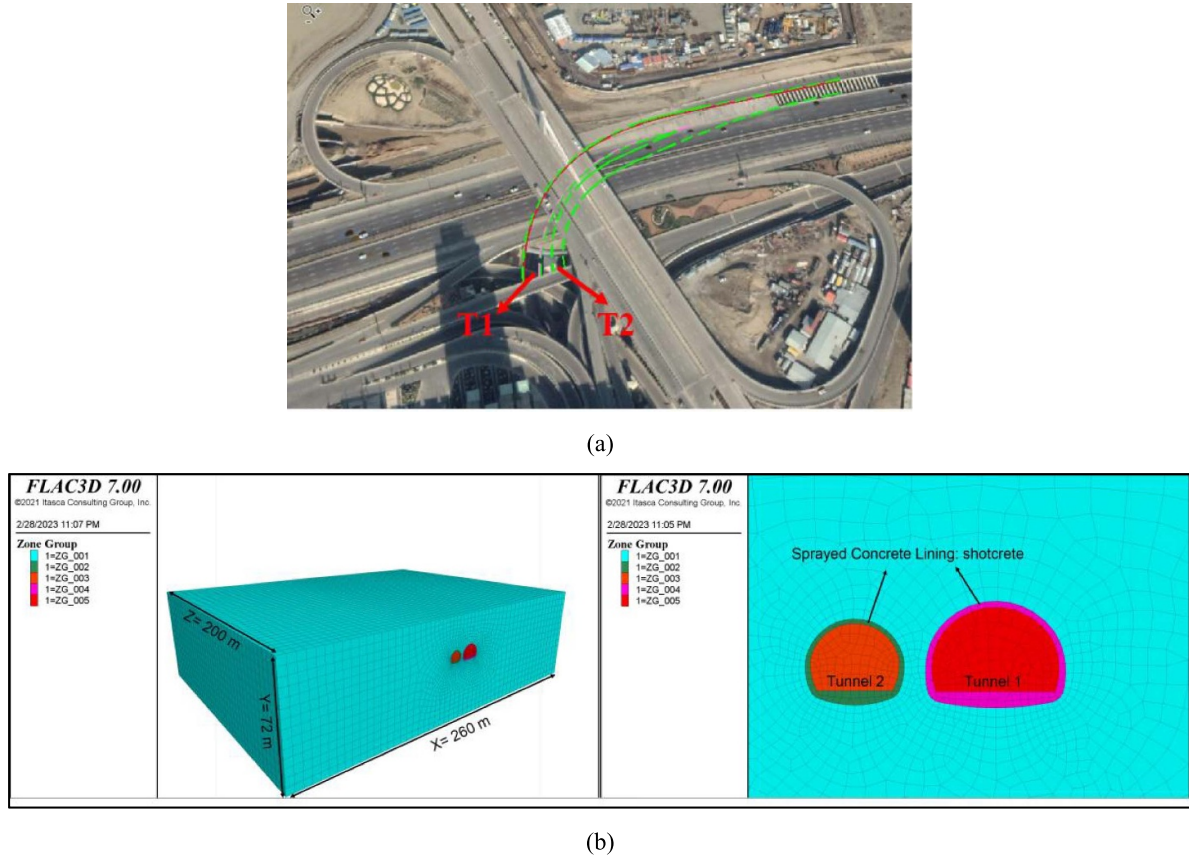
Figure 7. (a) Route plan for Iran Mall shopping tunnels (b) geometry, dimensions, and meshing of the Iran Mall tunnels numerical model.
