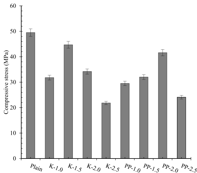
Figure 15. The compressive stress of the shotcrete reinforced with fibres.
