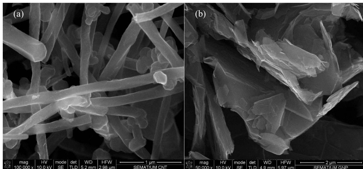
Figure 3. The structural features of carbon nanomaterials: (a) CNTs, (b) GNPs.
