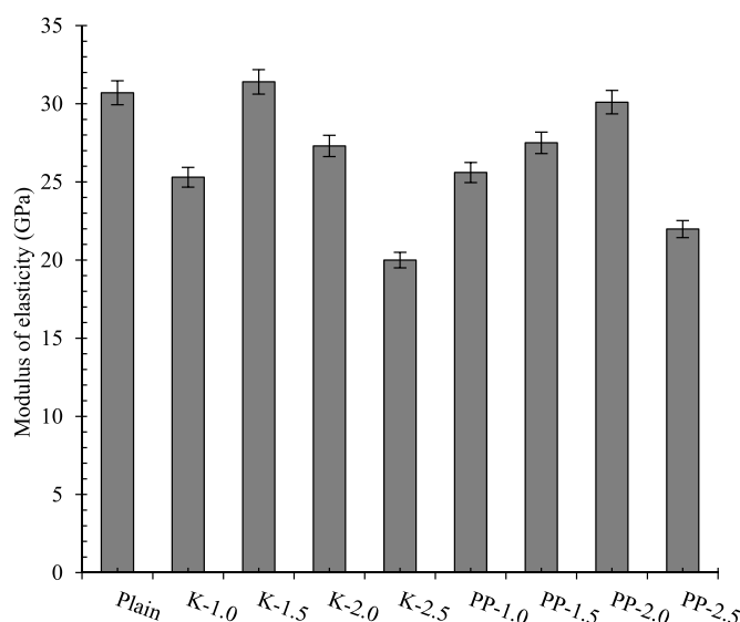
Figure 16. Elastic modulus of the shotcrete reinforced with fibres.
