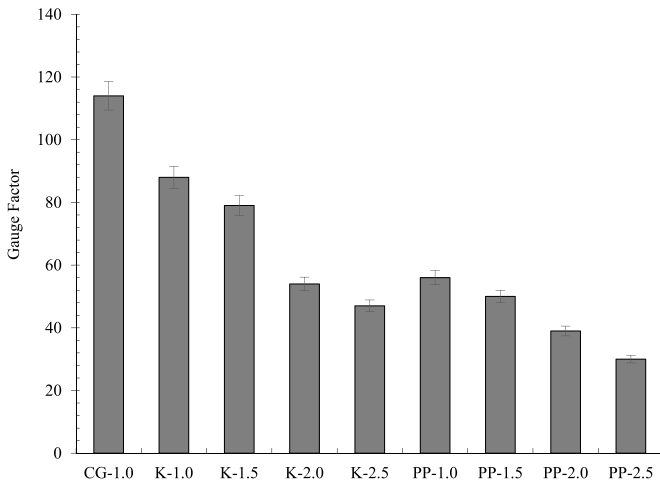
Figure 11. Gauge factors under compression cyclic loading for composites reinforced with Kenaf and PP fibres.
