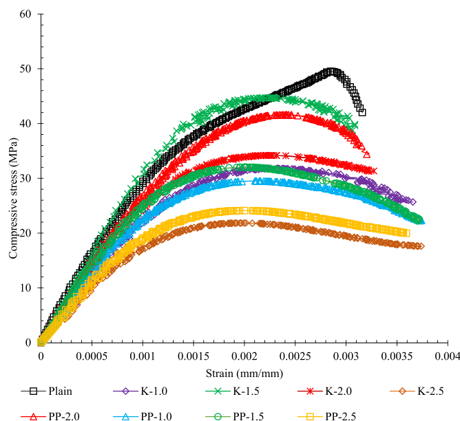
Figure 14. The stress-strain curves of the shotcrete reinforced with fibres.
