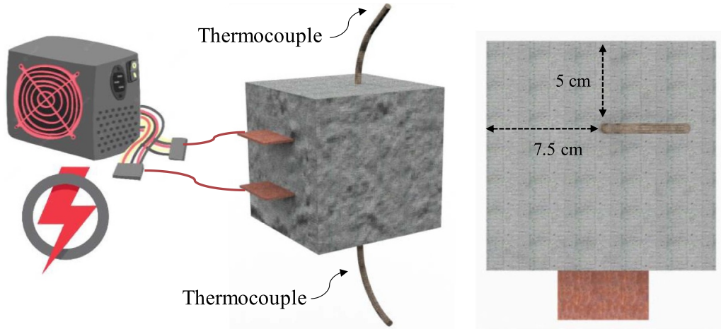
Figure 6. The experimental configuration employed for evaluating self-heating.
