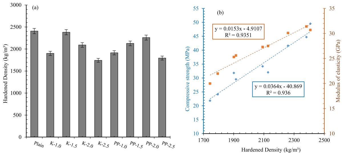
Figure 20. (a) The hardened density of the shotcrete reinforced with fibres, (b) correlation between hardened density, compressive strength, and modulus of elasticity.
