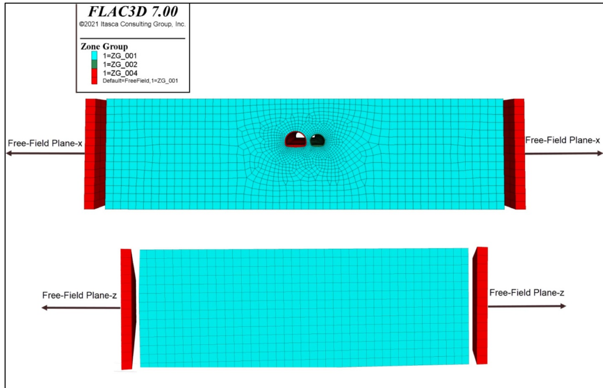
Figure 8. Dynamic boundary conditions in the lateral boundaries of the 3D model.
