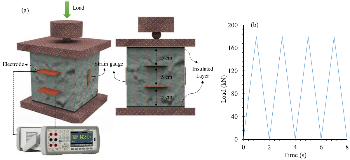
Figure 5. Test setup in piezoresistivity assessment: (a) specimen configuration, (b) cyclic load protocol.
