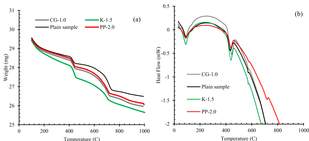
Figure 24. Thermal analysis of the specimen containing 1.5% Kenaf (K-1.5) and 2.0% PP (P-2.0): (a) TGA graphs, (b) DSC graphs.
