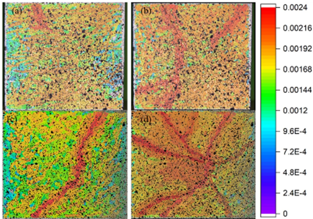
Figure 18. DIC analysis of the typical strain distribution at different stages of compression: (a) specimen K-1.5 (first crack), (b) specimen K-1.5 (a moment before the failure), (c) specimen PP-2.0 (first crack), (d) specimen PP-2.0 (a moment before the failure).
