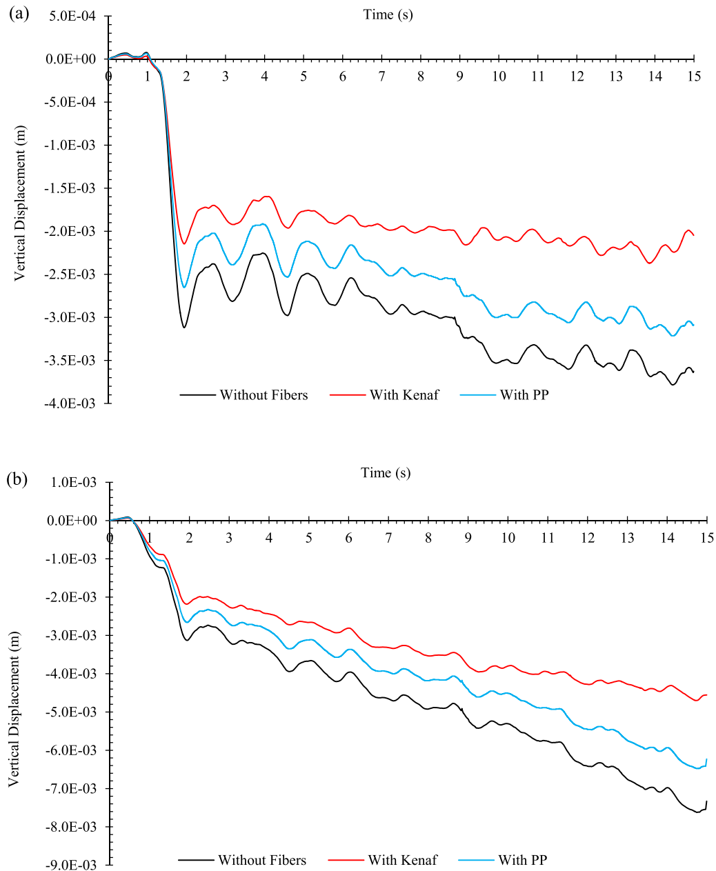
Figure 31. Vertical displacement curves of the tunnel shotcrete wall with different shotcrete types (settlement): (a) Tunnel 1 left wall, (b) Tunnel 2 right wall.
