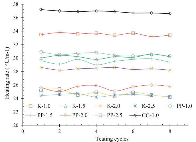
Figure 13. Average self-heating rate after 8 joule heating cycles.
