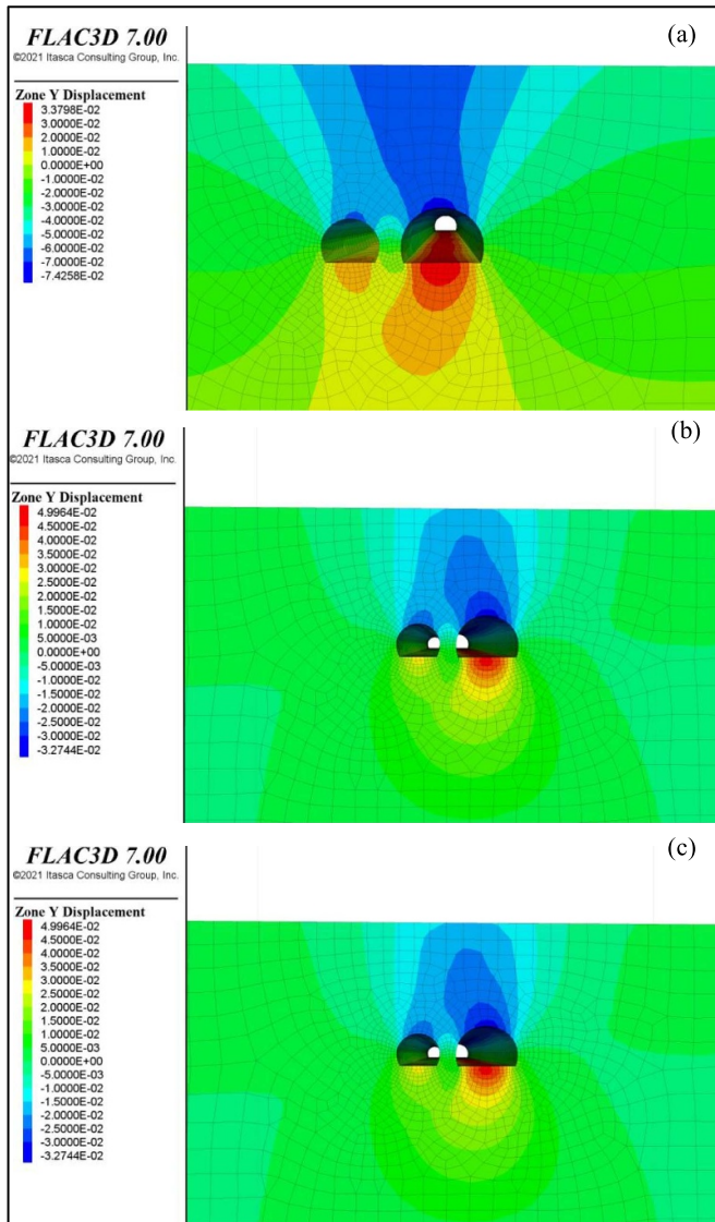
Figure 27. Vertical displacement contours of the tunnel numerical models with different shotcrete types (static loading): (a) without fibres, (b) with the optimum percentage of PP fibres (2.0%), (c) with the optimum percentage of Kenaf fibres (1.5%).
