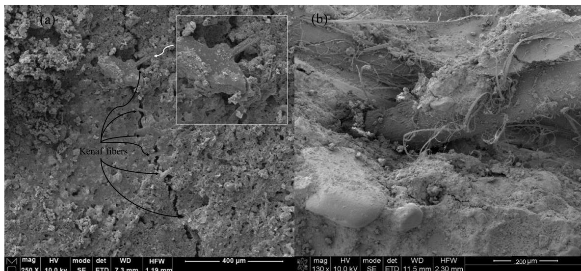
Figure 25. SEM morphology images of the cement-based composite reinforced with fibres: (a) Kenaf fibres, (b) PP fibres.
