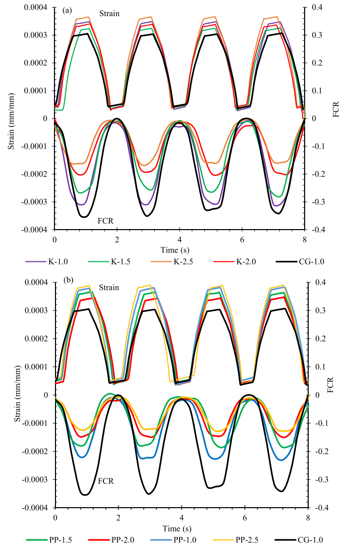
Figure 10. Strain–time–FCR curves under compression cyclic loading: (a) reinforced with Kenaf fibre, (b) reinforced with PP fibre.
