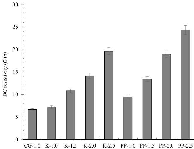
Figure 9. DC resistance of the composite reinforced with kenaf and PP fibres.
