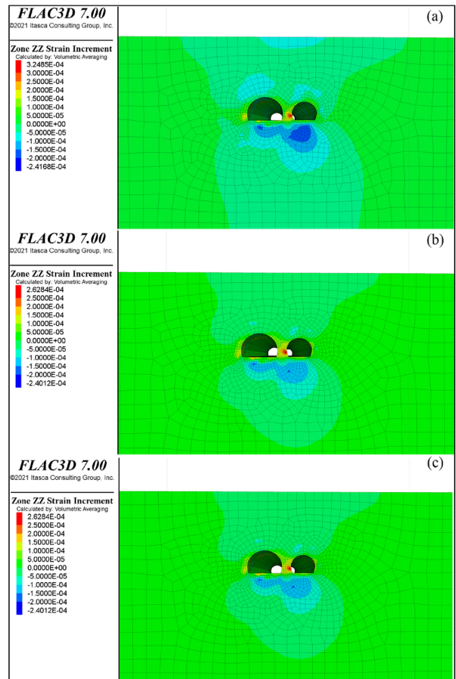
Figure 28. Vertical increment strain contours of the tunnel numerical models with different shotcrete types under static loading: (a) without fibres, (b) with the optimum percentage of PP fibres (2.0%), (c) with the optimum percentage of Kenaf fibres (1.5%).
