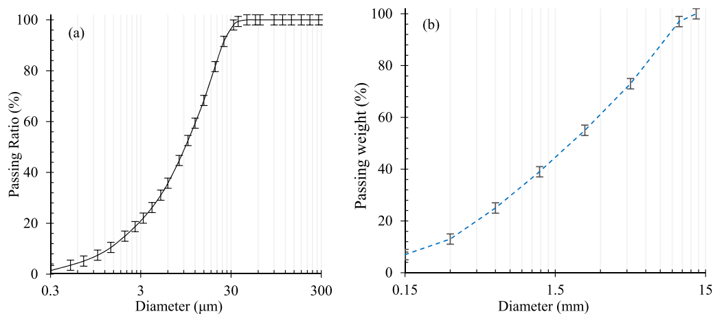
Figure 1. Particle size gradation curves of: (a) cement, (b) mixed aggregate (ASTM C136).
