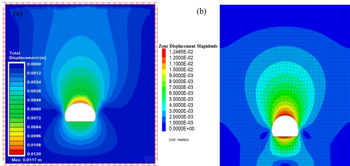
Figure 26. Final displacements after the tunnel enlargement of the preliminary 2D analysis in the Otter Sandstone formation: (a) numerical model of the masonry tunnel conducted by Atkinson et al [77] (Reprinted from Atkinson et al [77] Copyright 2021, with permission from Elsevier), (b) numerical model for verification.
