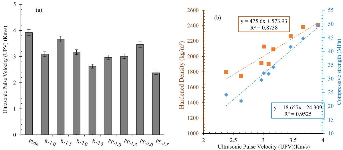
Figure 22. (a) Ultrasonic pulse velocity (UPV) of the shotcrete reinforced with fibres, (b) correlation between UPV, hardened density, and compressive strength.
