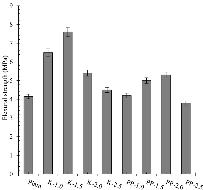
Figure 19. Flexural strength of the shotcrete reinforced with fibres.
