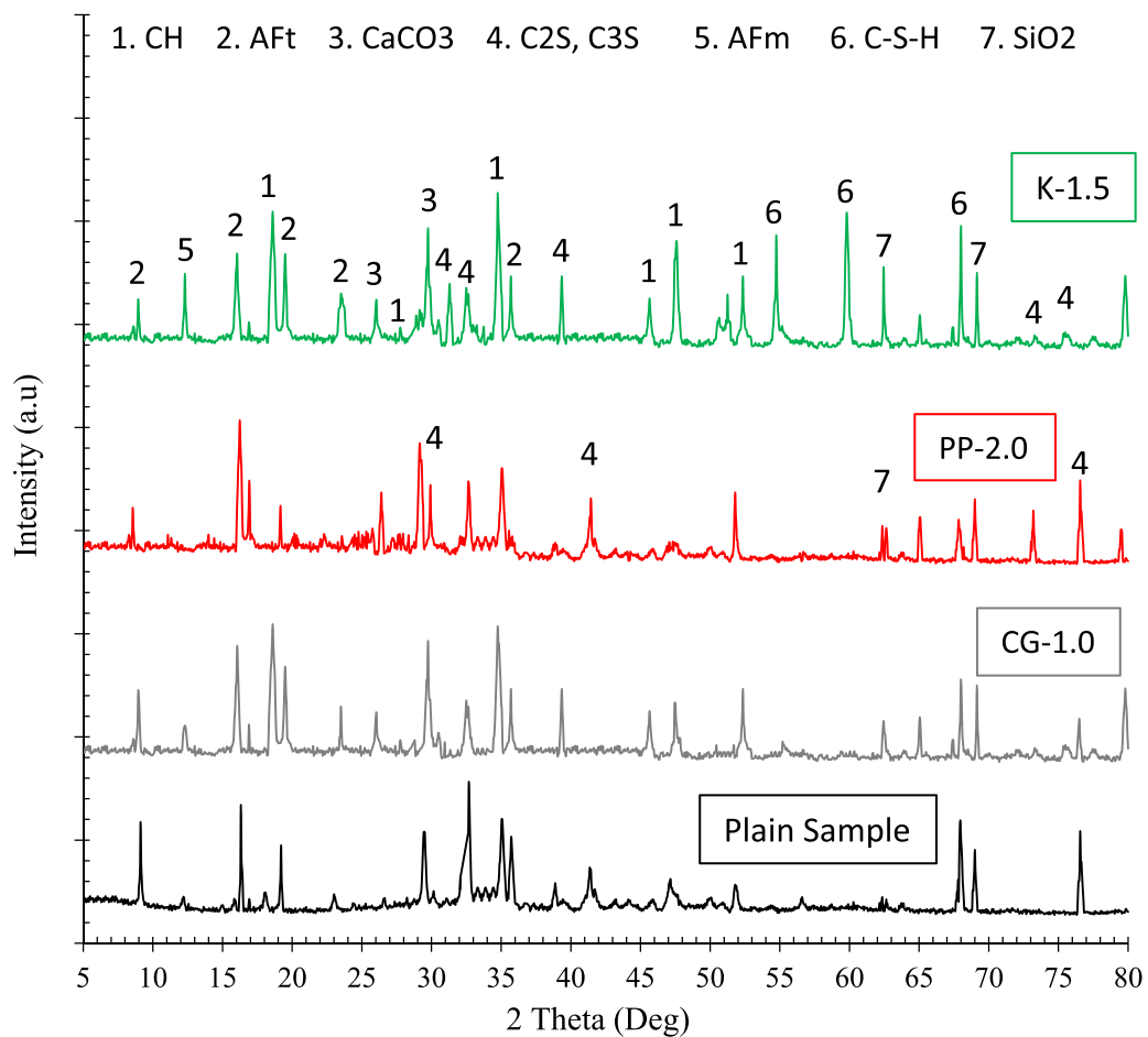
Figure 23. XRD spectra for the specimen reinforced with 1.5% Kenaf (K-1.5) and 2.0% PP (P-2.0).
