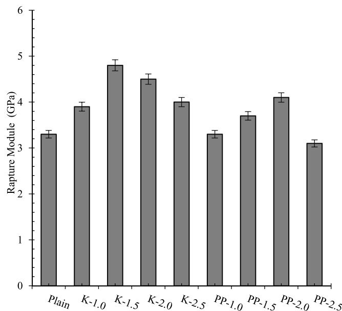
Figure 17. Rupture modulus of the shotcrete reinforced with fibres.
