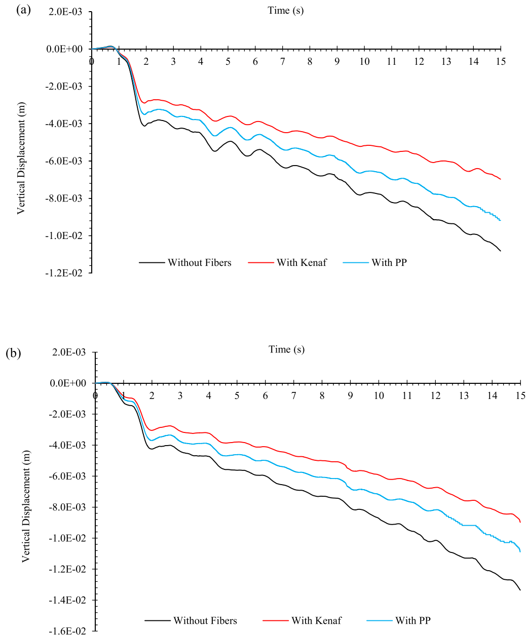
Figure 30. Vertical displacement curves of the tunnel shotcrete crown with different shotcrete types (settlement): (a) Tunnel 1 crown, (b) Tunnel 2 crown.
