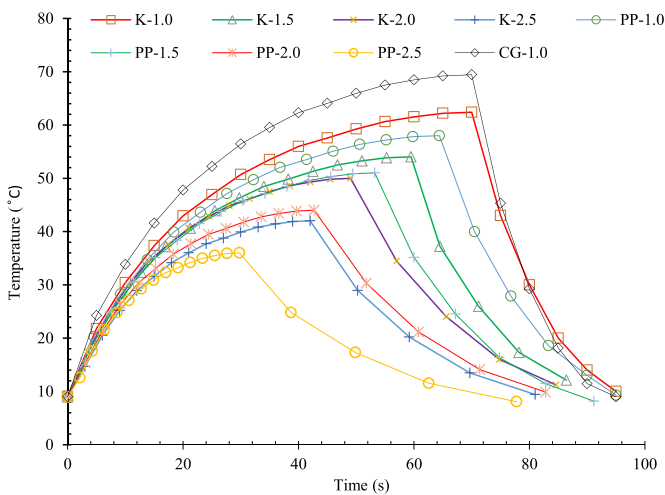
Figure 12. Temperature time histories of the composites reinforced with Kenaf and PP fibres.
