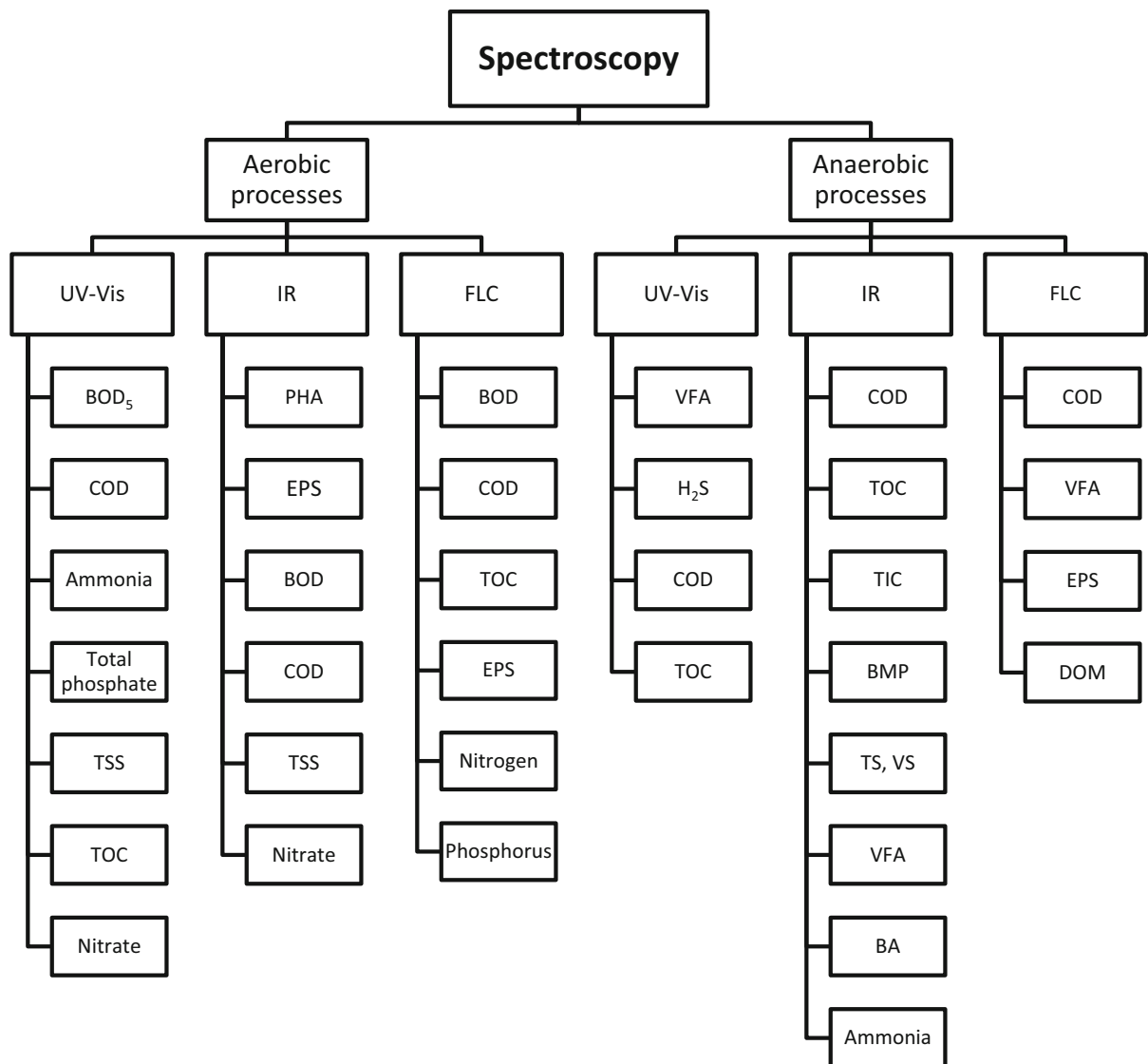
Fig. 1 Schematic representation of the spectroscopy techniques discussed in this review with the relevant parameters evaluated in each case
