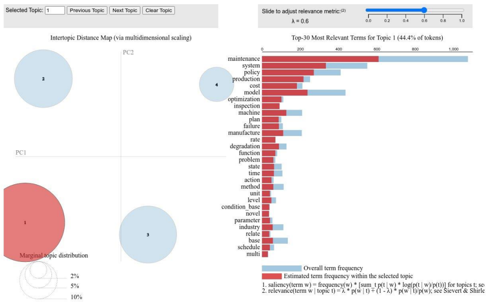
Figure 7. Intertopic Distance Map and the list of the Top-30 most relevant terms in topic 1 (2019-2023).
