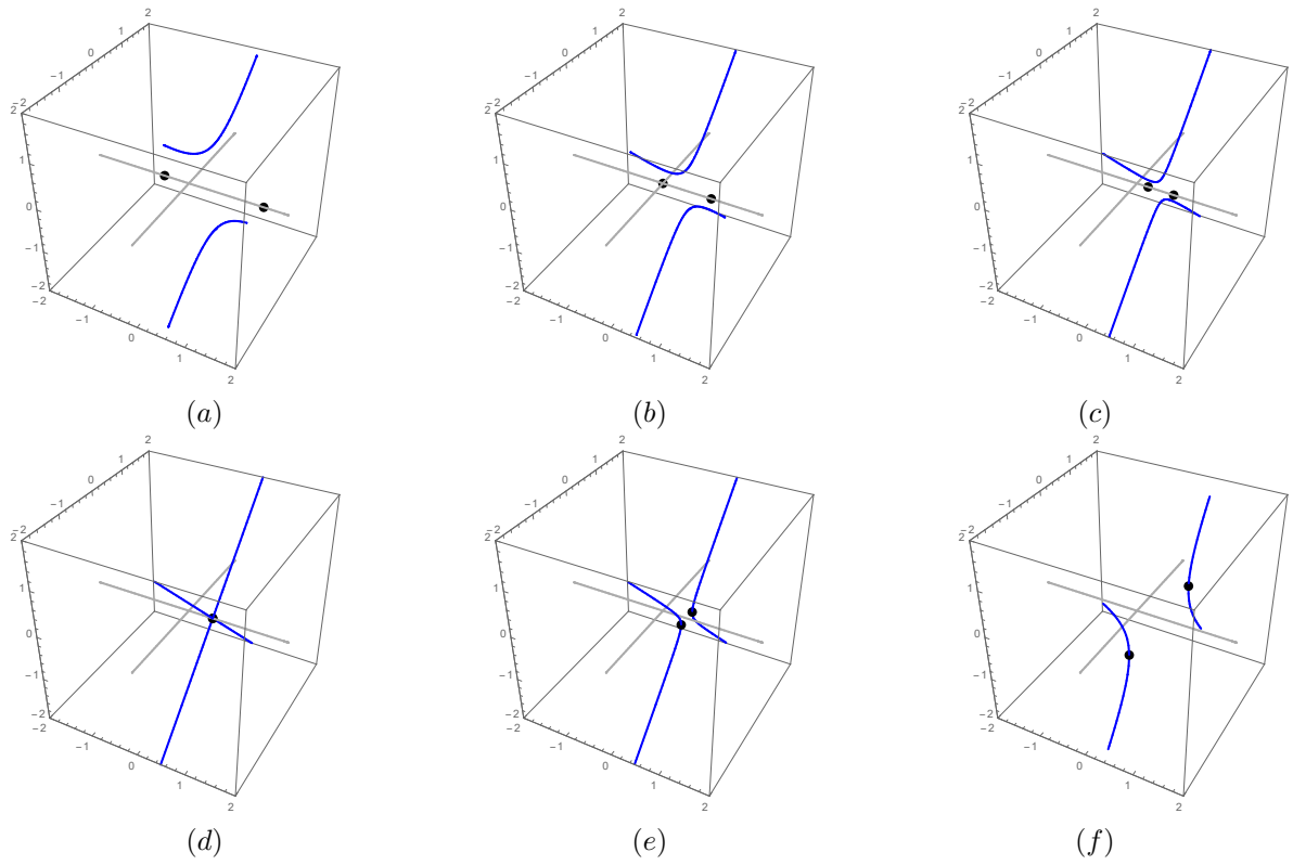
Figure 1: Plots, in the hyperplane q_3 = 0 , of the sets of fixed points corresponding to the case c = c_0 \in \mathbb{R} ; the real and complex fixed points are identified with black points and the fixed points not in \mathbb{C} form the blue lines; the gray lines represent the real and imaginary axes. (a) c_0 = -0.8 ; (b) c_0 = 0.0 ; (c) c_0 = 0.18 ; (d) c_0 = 0.25 ; (e) c_0 = 0.3 and (f) c_0 = 1.7 .
