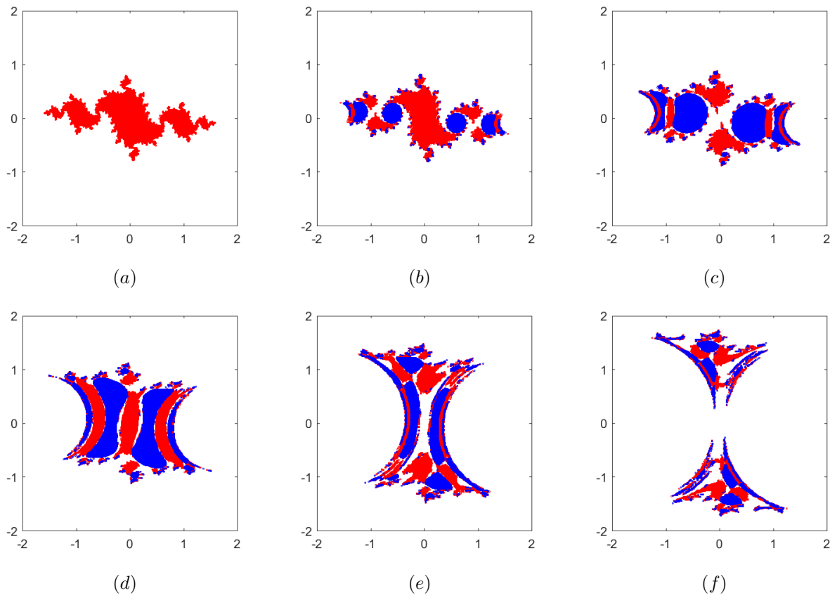
Figure 2: Plots, in different planes parallel to the complex plane, of the basins of attraction of the 2-cycle \mathcal{C}_2 (red) and of the (1,2)-set cycle \mathcal{C}_{1,2} (blue). (a) q_2 = 0 ; (b) q_2 = 0.2 ; (c) q_2 = 0.4 ; (d) q_2 = 0.8 ; (e) q_2 = 1.25 and (f) q_2 = 1.55 .
