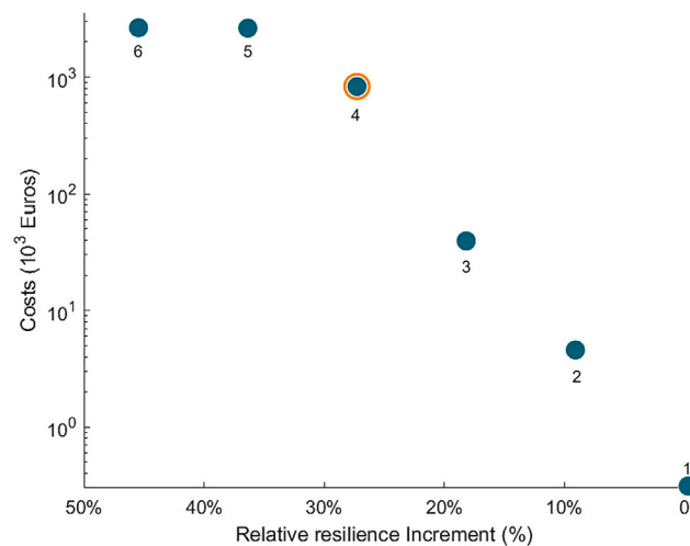
Fig. 6. Pareto Front with the optimal intervention strategies: Trade-offs between resilience increment and costs.
