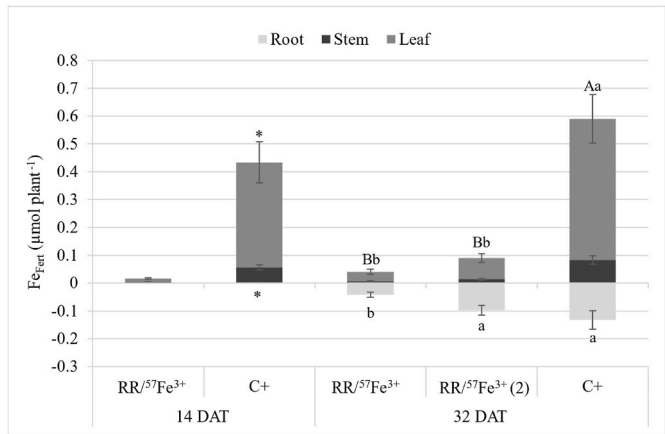
Fig. 5. Distribution of labeled ^{57}Fe ( Fe_{Fert} ) between plant organs for both samplings (14 and 32 DAT). Treatment of plants: please see the legend of Fig. 1. Mean \pm standard. Different superscript letters denote significant differences among the treatments according to Duncan's test p < 0.05 , ns: no significant differences. Capital letters correspond to the leaves. *denotes significant differences based on the Student's test ( p < 0.05 ).
