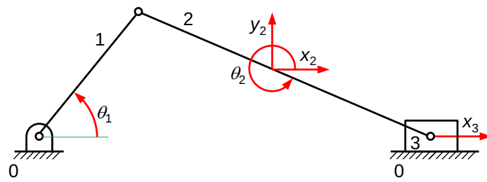
Fig. 4. Planar slider-crank mechanism.
