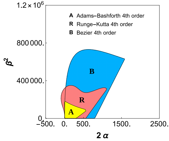
Fig. 3 Comparison between stability regions of Bezier, Adams-Bashforth and Runge-Kutta methods of order 4 with the same computational cost
