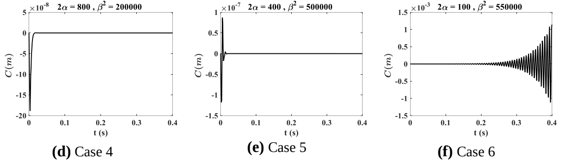
Fig. 7 Error of the 1st constraint equation with different Baumgarte parameters
