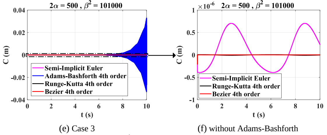
Fig. 9 Influence of the values of \hat{\alpha} and \hat{\beta} on the error of the 1st constraint equation for different numerical methods
