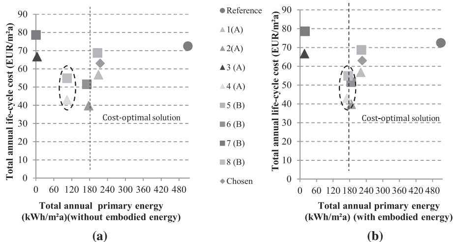
Figure 5. Results for the total primary energy (a) without embodied energy and (b) with embodied energy.
