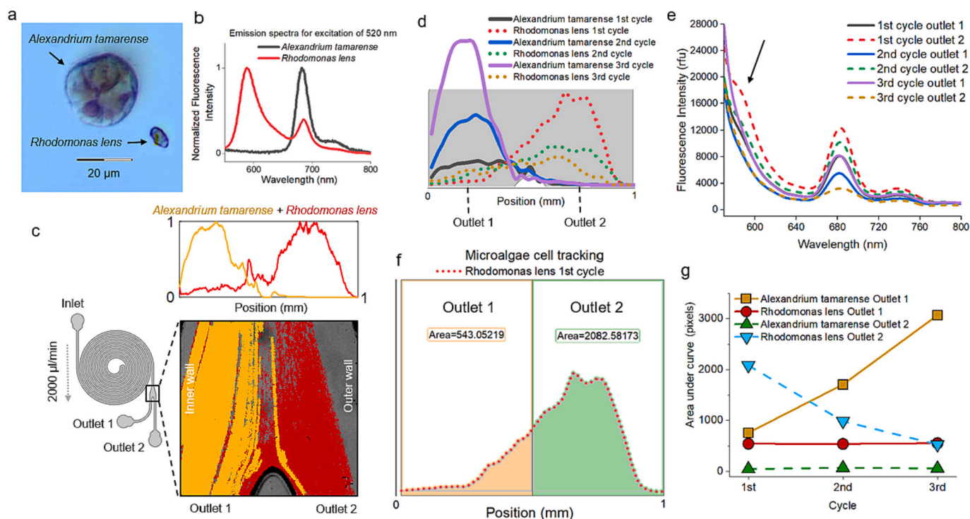
Fig. 7. a) Microscope image showing a size comparison between Alexandrium tamarensis (yellow) and Rhodomonas lens (red) (bar scale = 20 \mu m); b) normalized emission spectra excited at 520 nm for Alexandrium tamarensis and Rhodomonas lens . c) Visual representation of Alexandrium tamarensis and Rhodomonas lens tracking at the outlet region of the spiral; d) Alexandrium tamarensis and Rhodomonas lens trajectory at the outlets for the 3 cycles; e) Fluorescence emission spectrum excited at 520 nm for the sample mixture. f) Method to obtain the degree of isolation of species using the area under curve of the tracking plot of panel d. In this case, an example showing the Rhodomonas lens split between both outlets for the 1st cycle (details in Fig. S2 of section S3 of supplementary material); g) graph comparing the normalized area distribution under the curve at each outlet for both species across the 3 cycles. (For interpretation of the references to colour in this figure legend, the reader is referred to the web version of this article.)
