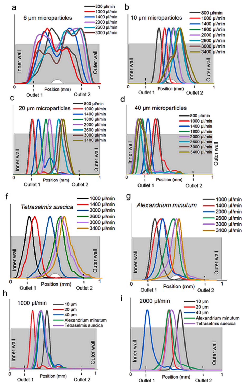
Fig. 4. Position for PS microparticles of a) 6 \mu\text{m} ; b) 10 \mu\text{m} ; c) 20 \mu\text{m} ; and d) 40 \mu\text{m} , f) Tetraselmis suecica and g) Alexandrium minutum , at the outlets for various flow rates, and position of microparticles and microalgae for fixed flow rates of h) 1000 \mu\text{l/min} and i) 2000 \mu\text{l/min} .
