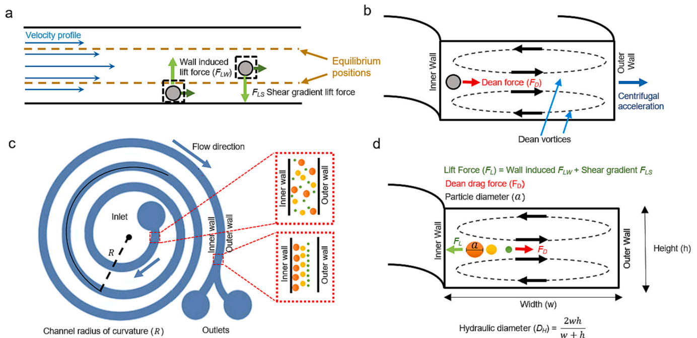
Fig. 1. a) (Top view parallel to flow direction) Representation of the net inertial lift forces composed by the shear gradient induced lift force and wall induced lift force (blue arrows represent the parabolic nature of the velocity profile) and b) (channel cross-section view perpendicular to flow direction) the Dean drag force in curved channels; c) schematic representation of the equilibrium position of different sized particles along the spiral and d) microchannel cross section showing the interaction between the net lift force ( F_L ) and the Dean drag force ( F_D ). (For interpretation of the references to colour in this figure legend, the reader is referred to the web version of this article.)
