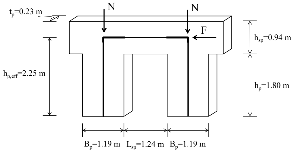
Figure 5. Schematic representation of the PS3 substructure according to the EF model.
