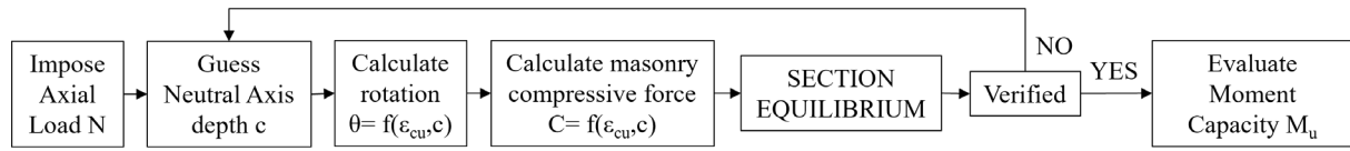
Figure 2. Calculation of the M-N domain through sectional analysis using the MBA approach.
