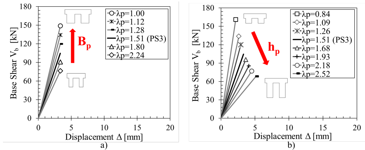
Figure 12. Capacity curves of the substructures when varying the (a) piers length B_p and (b) piers height h_p . Note: when the spandrel fails by shear, the lines represent only the yield limit.
