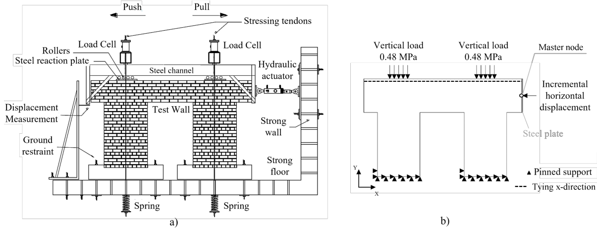
Figure 3. Benchmark tested substructure: (a) cyclic testing setup (adapted from Knox et al. [31]) and (b) sketch of the adopted boundary conditions.
