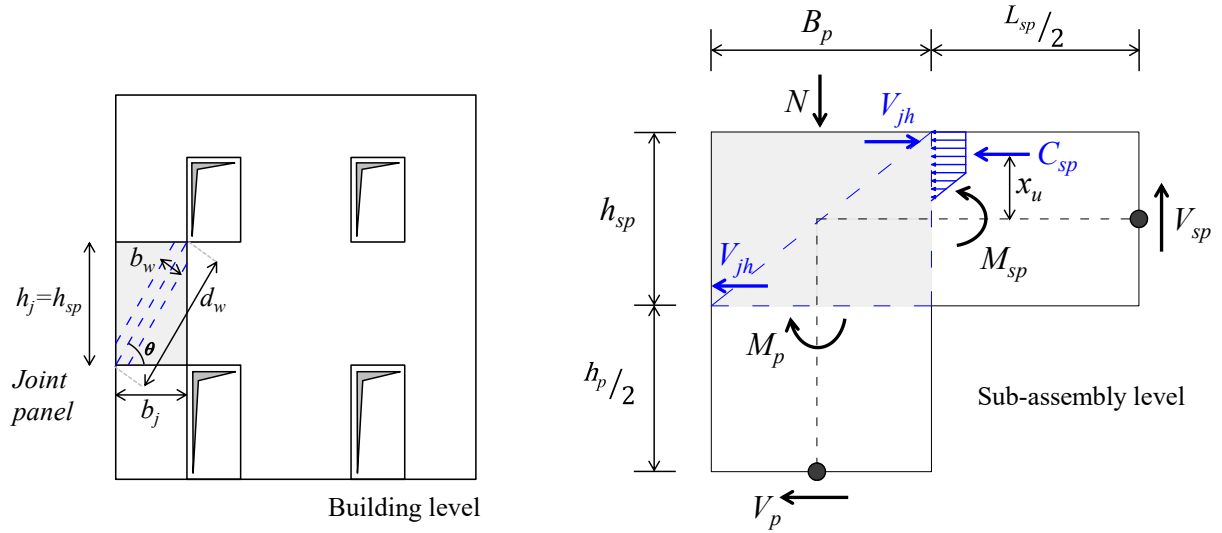
Figure 13. Schematization of the parameters to find the strength of a joint at a generic external subassembly (adapted from [20]).
