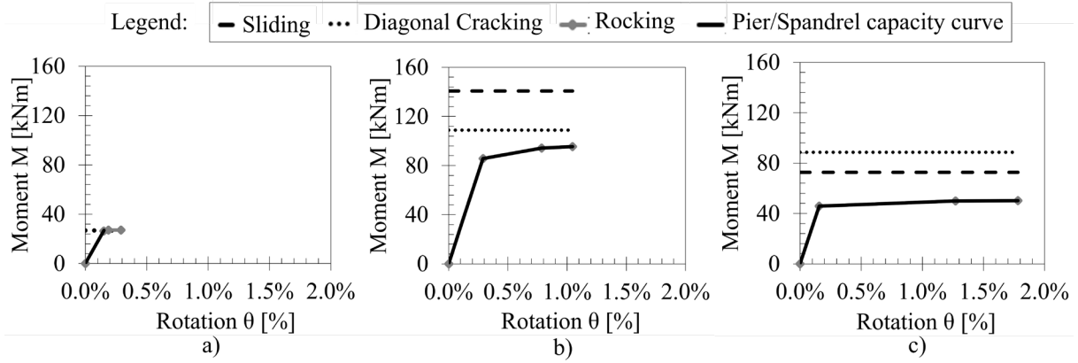
Fig. 7. Flexural and shear strength thresholds at the moment-rotation diagram for (a) spandrel (EPP-TR-TF model), (b) left pier (EPP-NTR model) and (c) right pier (EPP-NTR model).
