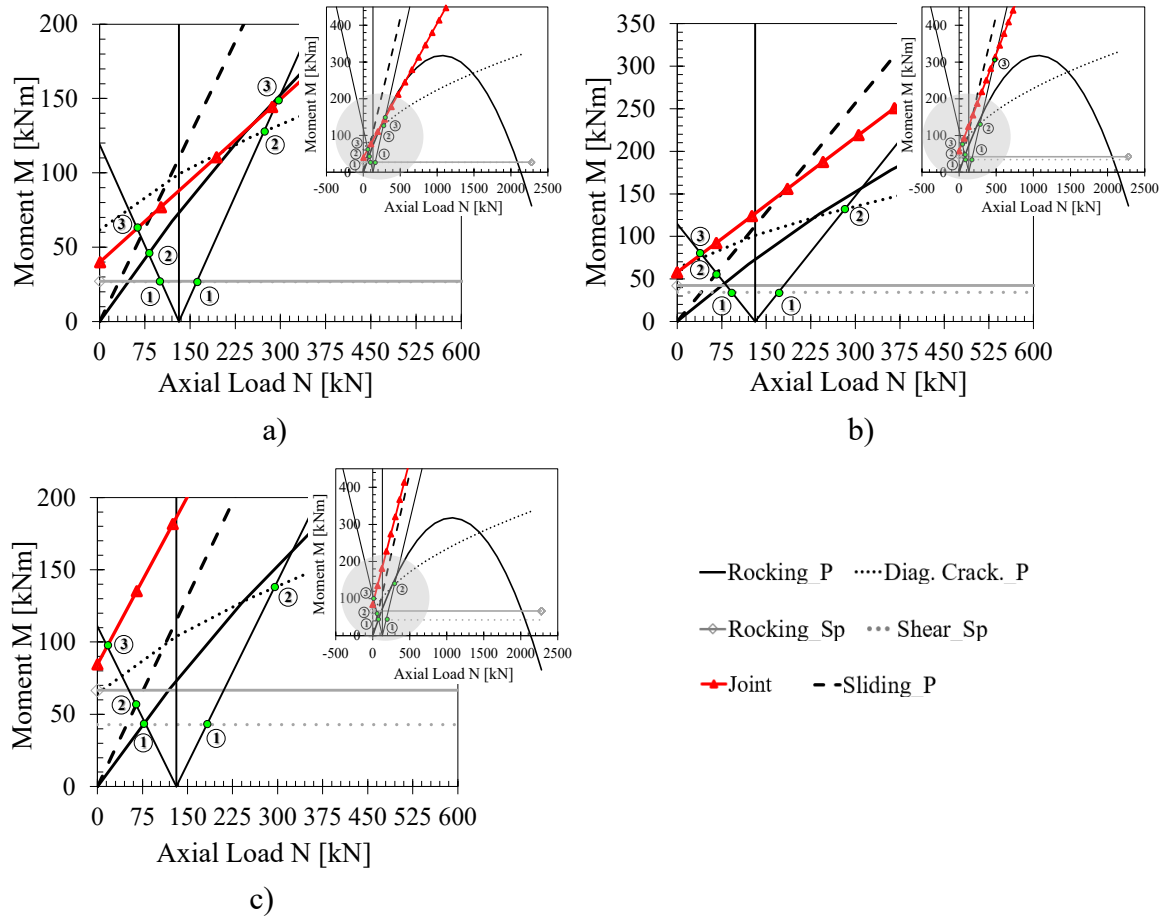
Figure 14. Pier M - N performance domains for subassemblies with an h_{sp} of (a) 0.94 m, (b) 1.20 m and (c) 1.50 m (circled numbers indicate the failure sequence events).
