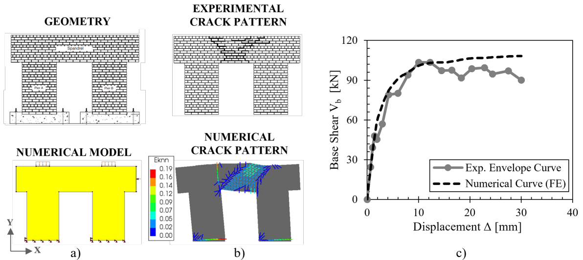
Figure 4. Simulation of the PS3 substructure: (a) geometry and FE model, (b) experimental and numerical crack patterns (normal crack strain) at the ultimate displacement and (c) numerical capacity curve against experimental envelope.
