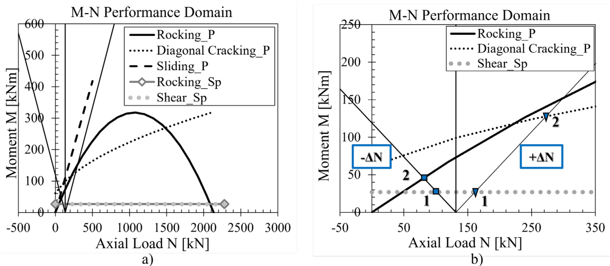
Figure 9. Frame analysis: (a) M-N performance domain; (b) zoom highlighting the sequence of failure events (■: right subassembly ( -\Delta N ), ▼: left subassembly ( +\Delta N )).
