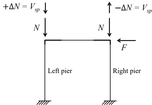
Figure 6. Frame subjected to horizontal load and gravity load with axial load variation.
