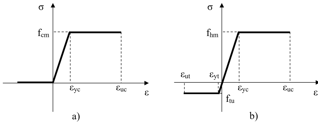
Figure 1. Stress-strain relationships: (a) elastic–perfectly plastic in compression and no-tensile resistant (EPP-NTR) for piers, and (b) elastic–perfectly plastic in compression and tensile resistant (EPP-TR) for spandrel.
