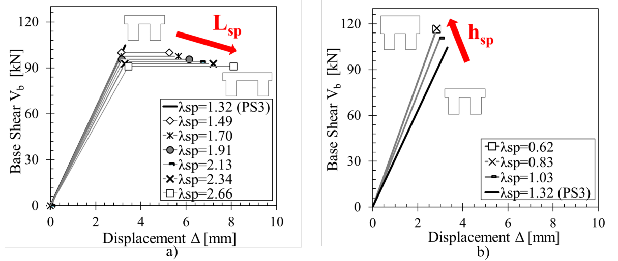
Figure 11. Capacity curves of the substructures when varying the (a) spandrel length L_{sp} and (b) spandrel height h_{sp} . Note: when the spandrel fails by shear, the lines represent only the yield limit.
