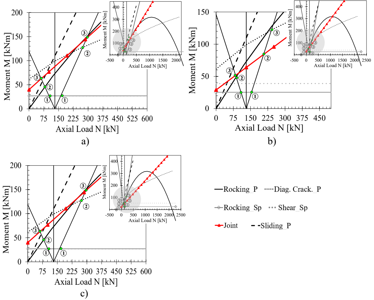
Figure 15. Pier M – N performance domains for subassemblies with an L_{sp} of (a) 1.24 m, (b) 1.80 m and (c) 2.50 m (circled numbers indicate the failure sequence events).
