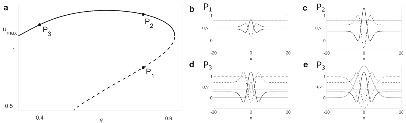
Fig. 2 a Bifurcation curve showing one-bump solutions of (1) with a Mexican-hat kernel (2) as the threshold parameter \theta is varied. Solid (dashed) lines represent stable (unstable) solutions. u_{\max} is the maximum of u over all x . (b–e) Examples of solutions at the points P_1 (unstable) and P_2 (stable) for \theta = 0.8 (dotted line) and P_3 (stable) for \theta = 0.4 (dotted line) are shown. Solid and dashed black lines represent u(x) and v(x) , respectively. For the solution at the point P_3 we show
