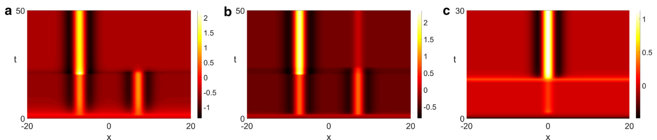
Fig. 13 ( a and b ) Retro-cueing task in the Amari model ( a ) and in the two-field model ( b ). Bumps were initially created with two inputs with A_{I_{1,2}} = 0.75 , \sigma_{I_{1,2}} = 1 , d_I = 1 . Later at time t = 20 an additional input with A_{I_1} = 2 , \sigma_{I_1} = 1 , d_I = 1 was applied to one of the memories. The kernel w is given by (2) with A_{ex} = 2 , A_{in} = 1 , \sigma_{ex} = 1.25 , \sigma_{in} = 2.5 and w_{inh} = 0.2 . Threshold \theta = 0.4 , K = 0 . ( c ) Recov-
