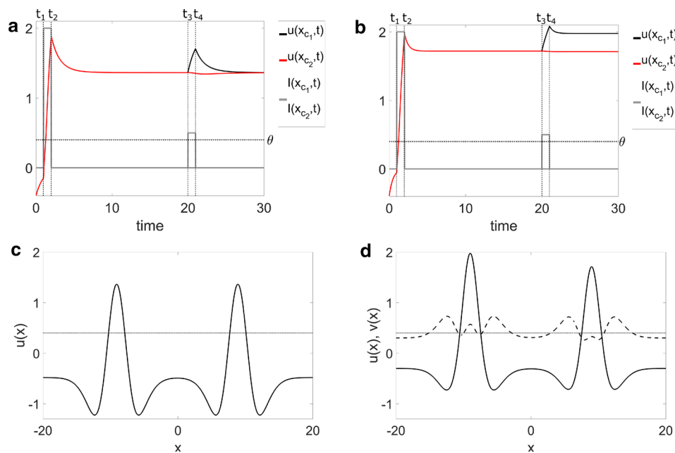
Fig. 12 Retro- cueing task in the Amari model ( a and c ) and in the two-field model ( b and d ). Bumps are created with two inputs (grey lines) with A_{I_{1,2}} = 2 , \sigma_{I_{1,2}} = 1 , d_I = 1 applied simultaneously at time t_1 = 1 at positions x_{c1} = -9 and x_{c2} = 9 . At a later time t_3 = 20 , an additional weak input with A_{I_1} = 0.5 , \sigma_{I_1} = 1 , d_I = 1 is applied to
