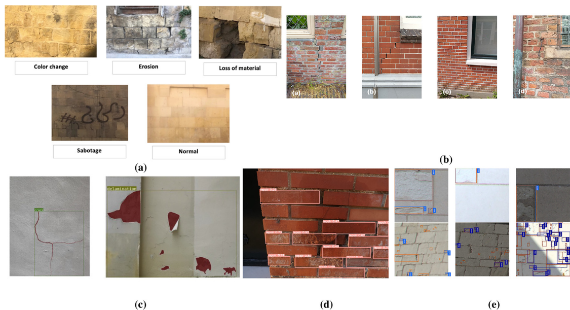
Fig. 5. a) CNN deployed by Samhouri et al. [59] for façade damages in “Al-Salt” in Jordan, b) masonry surface defects considered by Dais et al. [64], c) sample façade defects (e.g. crack and delamination) [62], d) AI-system for façade bricks to indicate need to clean or repair [66] (red bounding box and red text showing repair label), e) correct (first row) and incorrect (second row) AI-assisted models results for tiny degradation on surfaces [63] (red bounding box showing predictions with confidence score in blue text).
