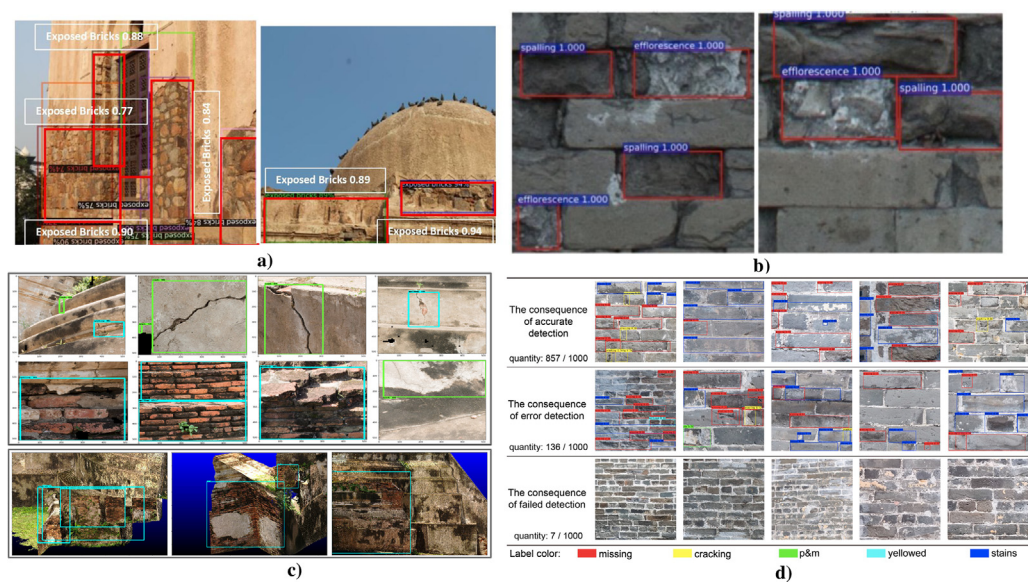
Fig. 4. Examples of AI-assisted visual inspection systems for surface defects: a) employing YOLO for detecting surface damages in Dadi-Poti case study [37], b) detecting damages for efflorescence and spalling [39], c) Faster R-CNN model for detecting spalling (light blue bounding box) and cracks (light green bounding box) [52], d) categorizing five types of damages for CH in Macau [53].
