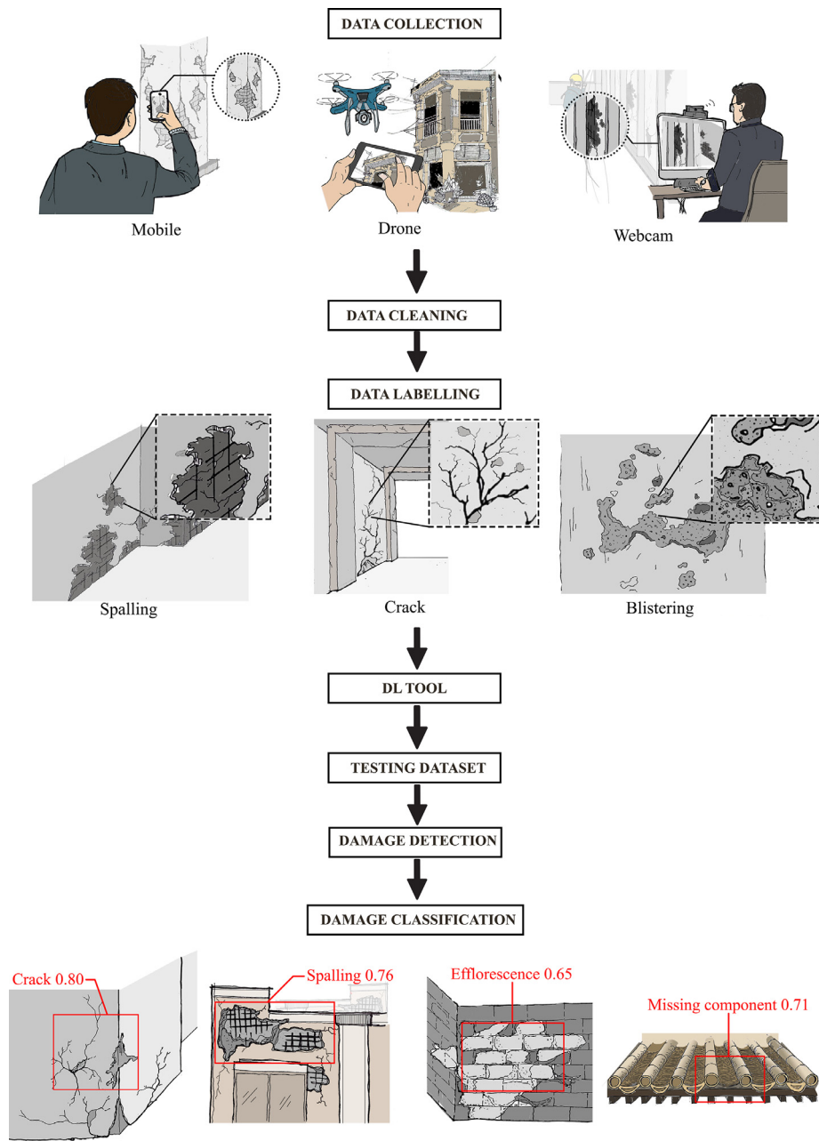
Fig. 2. Flowchart of AI-assisted inspection process (Sub figures adapted from Zou et al. [35], Li and Liu [6], Mansuri and Patel [36], Mishra et al. [37] and Wang et al. [38,39]).
