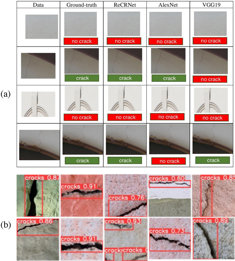
Fig. 6. a) An AI-based tool named ReCRNet deployed by Reis and Khoshelham [68] for crack detection in CH buildings, b) YOLO-based DL-model for detecting cracks in CH buildings in Bhubaneswar India [71].
